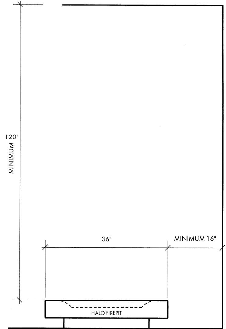
CLEARANCES to COMBUSTIBLE MATERIALS
